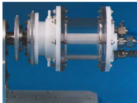
The major component of the Bioreactor Demonstration System is the transparent rotating wall vessel. It resides in a locker containing nutrient media bags and an oxygenator, plus associated plumbing to operate the system.
