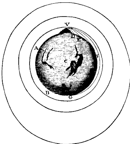
Newton's Thought Experiment: A cannonball fired with enough force could fall endlessly around (or orbit) the Earth.
