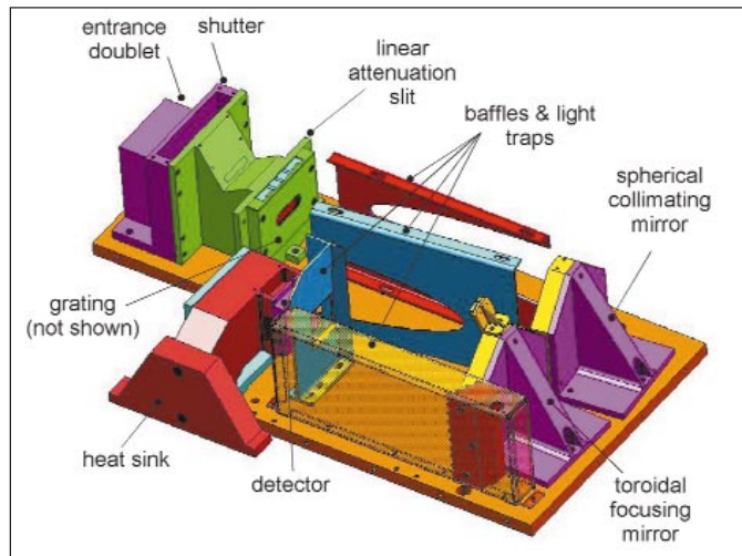
SOLSE instrument is a Czerny-Turner imaging spectrometer.
