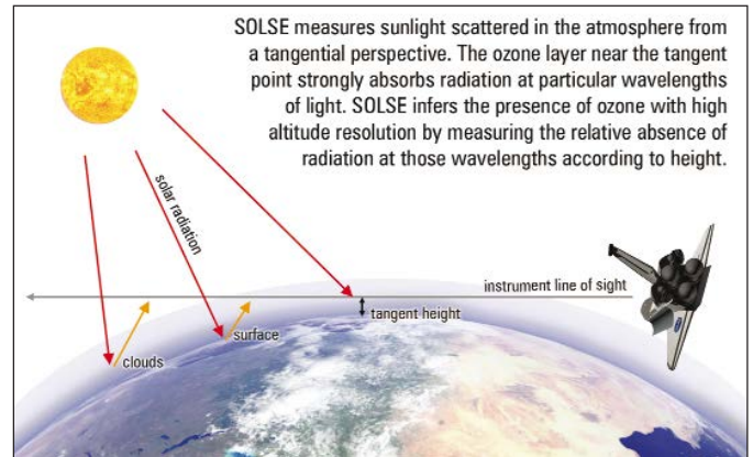
This illustration shows how ozone is seen using light scattered from the Earth's limb.
